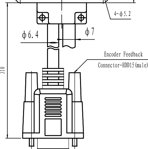
EncoderFeedBack Cable wires Assignment
